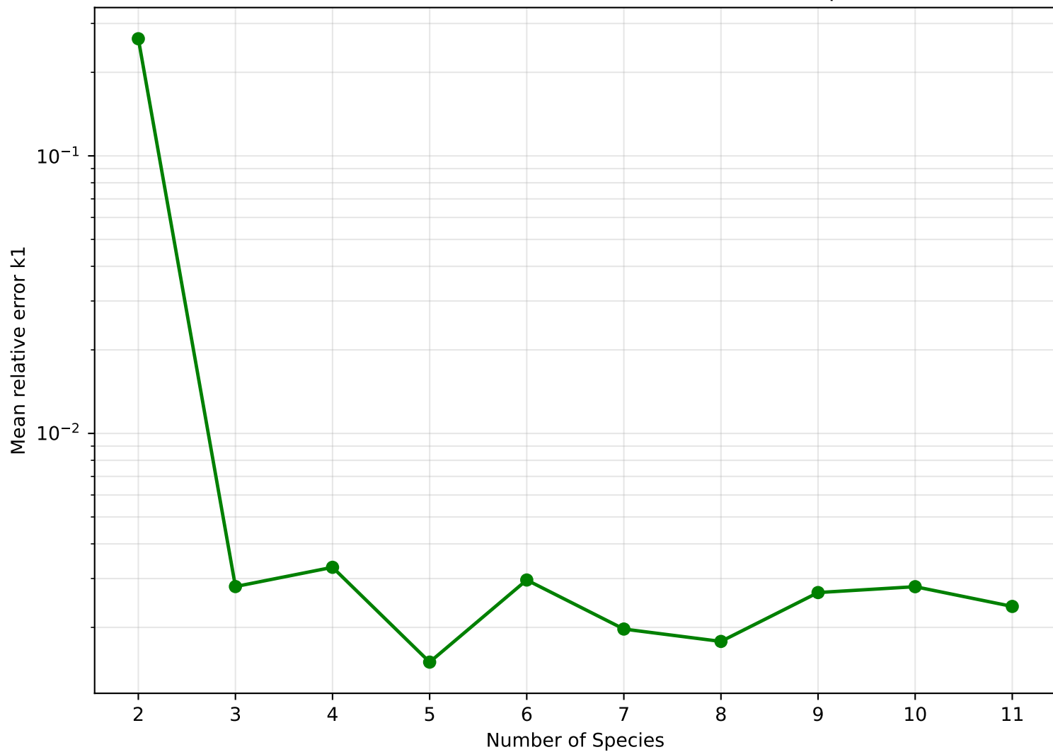
30, 30, 30 — Mean relative error k1 vs number of species
